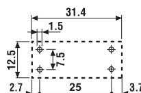
45.31...0610 (1 NO/SPST-NO)
